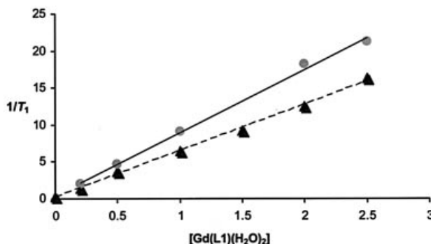
Figure 4. A plot of concentration of [Gd(DO3A\text{-}Pr\text{-}ATP)(H_2O)_2] vs. 1/T_1 in the presence (●) and in the absence (▲) of \beta -cyclodextrin.
