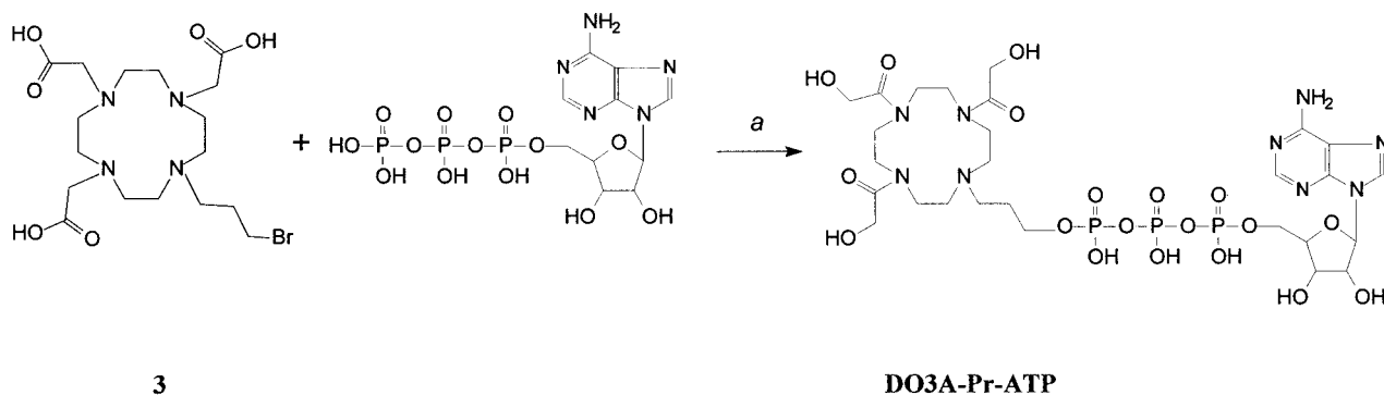
Scheme 2. Synthesis of DO3A-Pr-ATP. Conditions: (a) water, room temp., 36 h.
