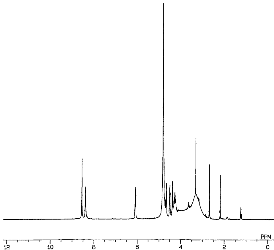
Figure 2. ^1\text{H} NMR spectrum of 10-[3-(adenosine 5'-triphosphate)oxypropyl]-1,4,7-tris(carboxymethyl)-1,4,7,10-tetraazacyclododecane (DO3A-Pr-ATP).
