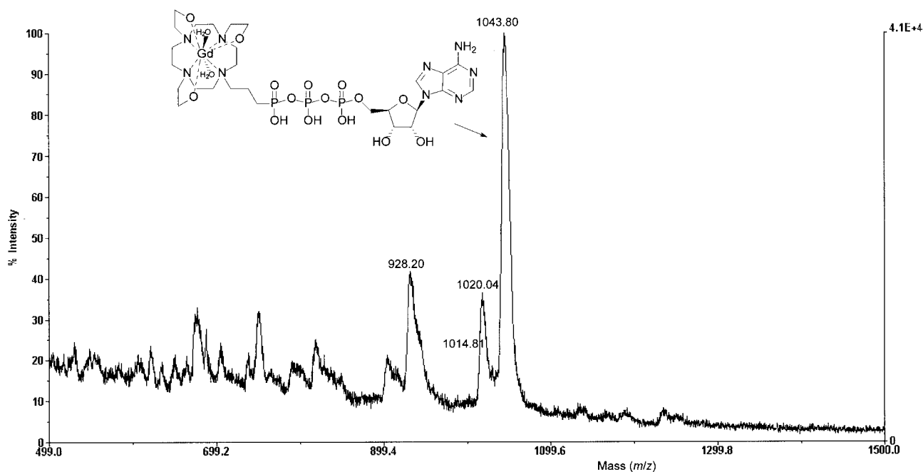
Figure 3. MALDI TOF mass spectrum of [\text{Gd}(\text{DO3A-Pr-ATP})(\text{H}_2\text{O})_2] ( 4 ).
