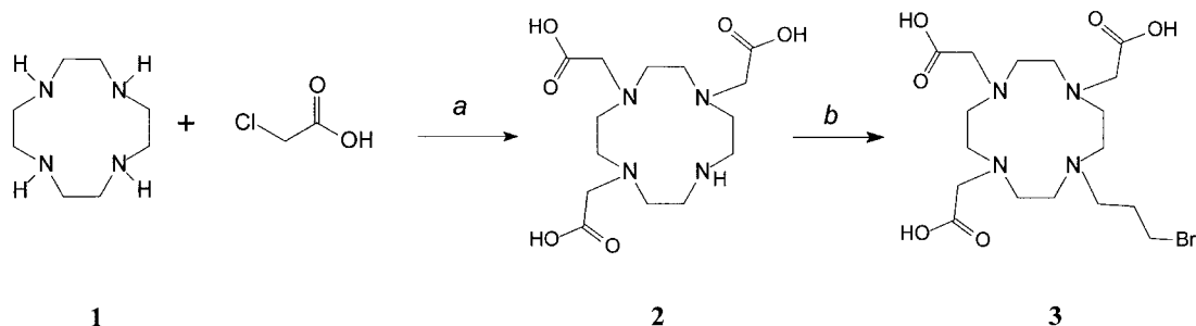
Scheme 1. Synthesis of linker appended DO3A. Reagents and conditions: (a) -4^\circ\text{C} , H 2 O, NaOH, pH 10; (b) 1,3-dibromopropane, DMF/water, triethylamine.
