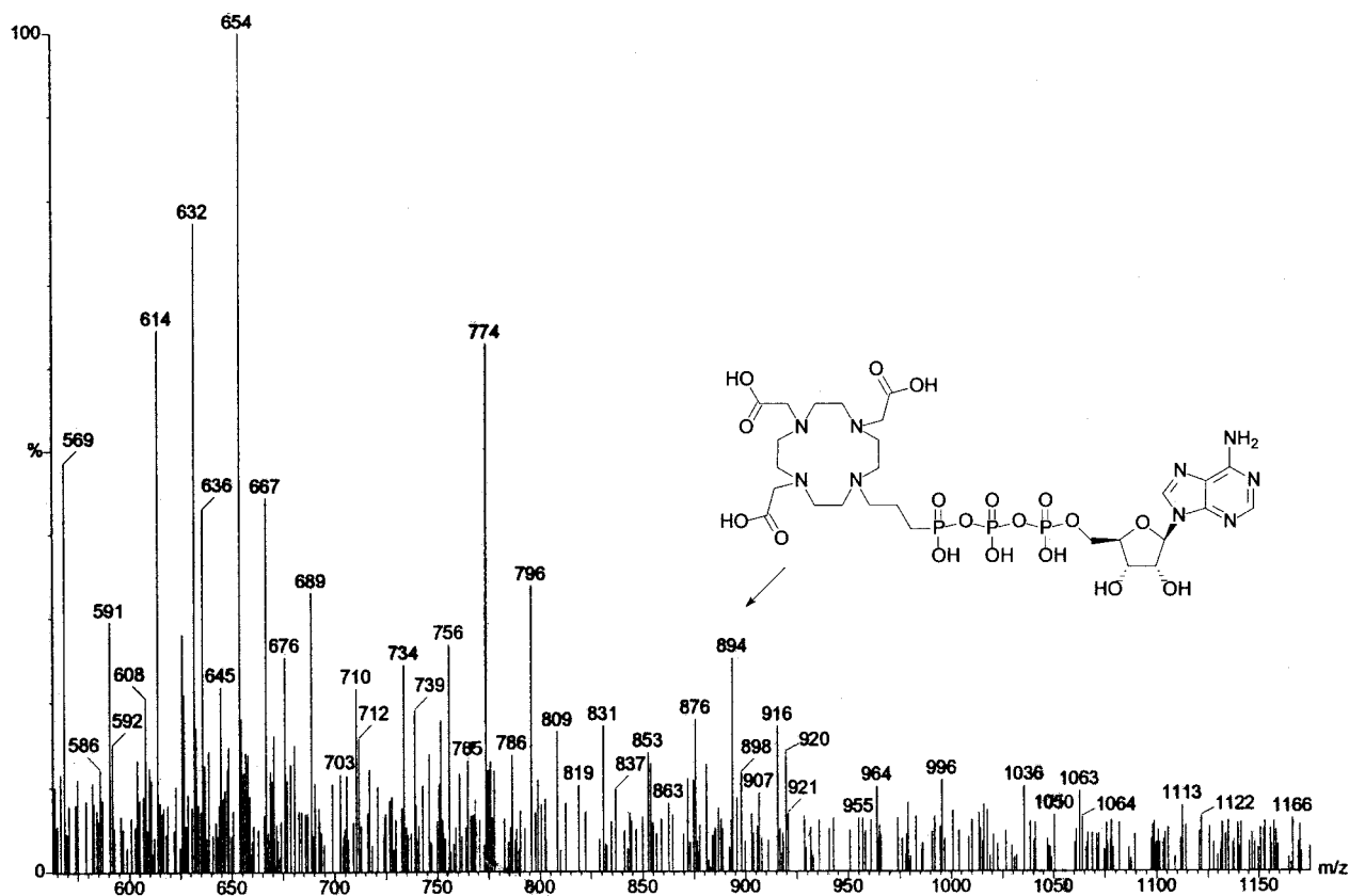
Figure 1. ESI mass spectrum of 10-[3-(adenosine 5'-triphosphate)oxypropyl]-1,4,7-tris(carboxymethyl)-1,4,7,10-tetraazacyclododecane (DO3A-Pr-ATP).
